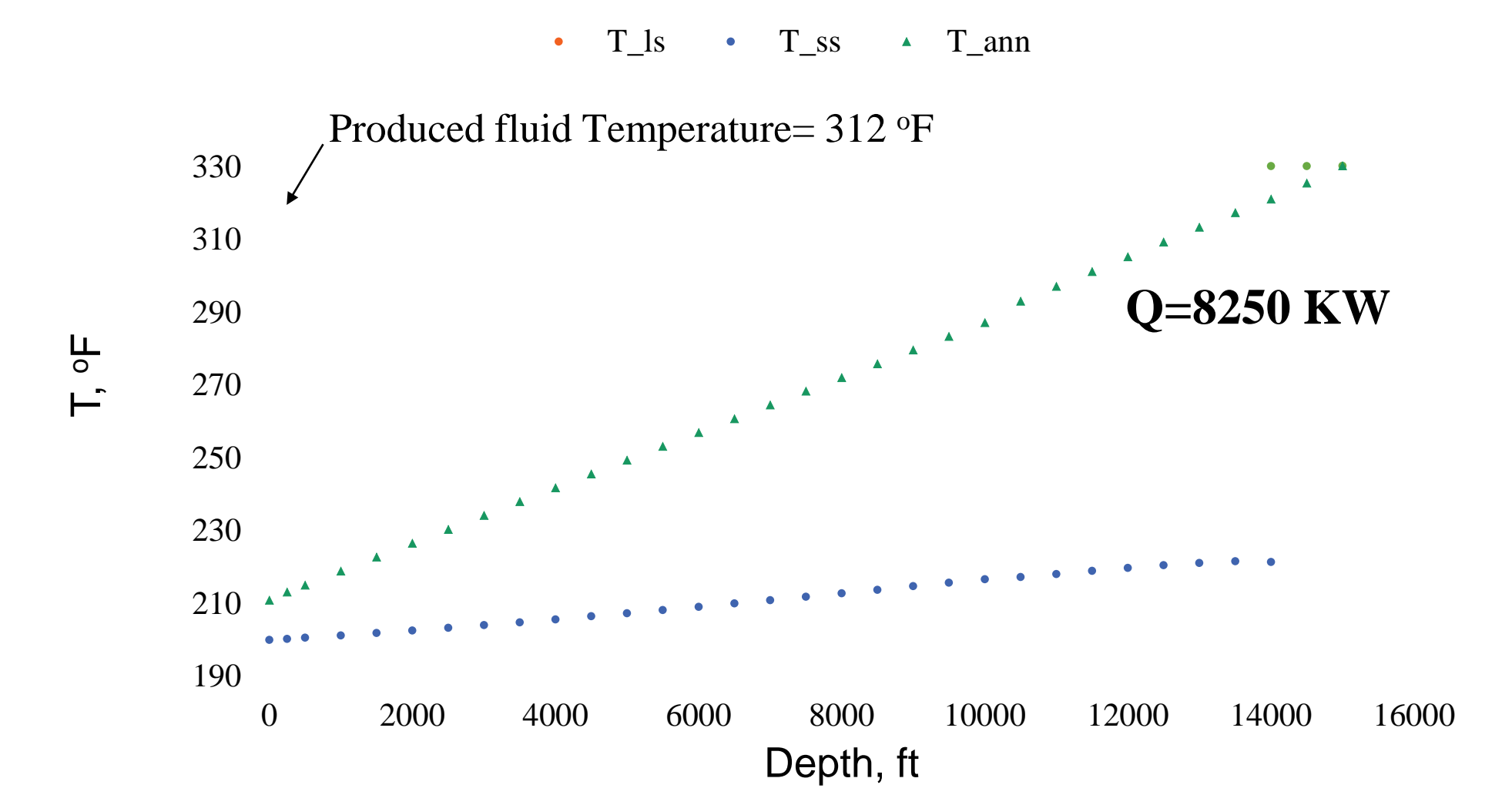
Fig 3. Fluid temperature in three conduits at q=500 gpm and N_2 depth=14000 ft at Q=8250 KW
